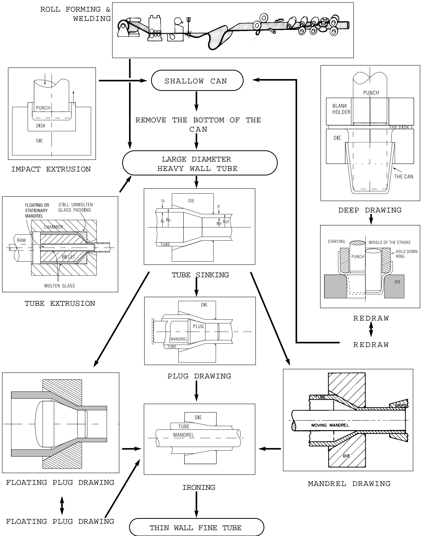
FIG. 1 SCHEMATIC ALTERNATE PASS REDUCTION SCHEDULES FOR TUBE MAKING
